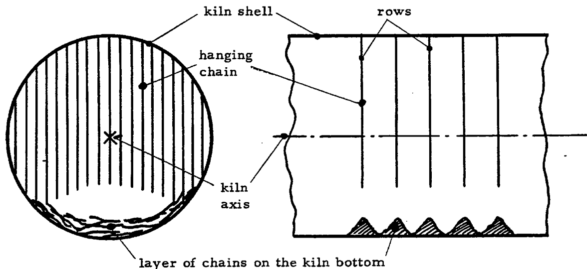
Figure 2: Straight Curtain
